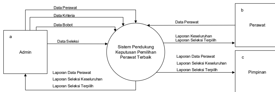
Gambar 2. Desain Context Diagram
